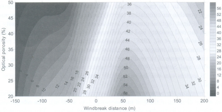
Fig. 5. Wind speed reduction (in %) at different distances from the windbreak depending on the OP.
